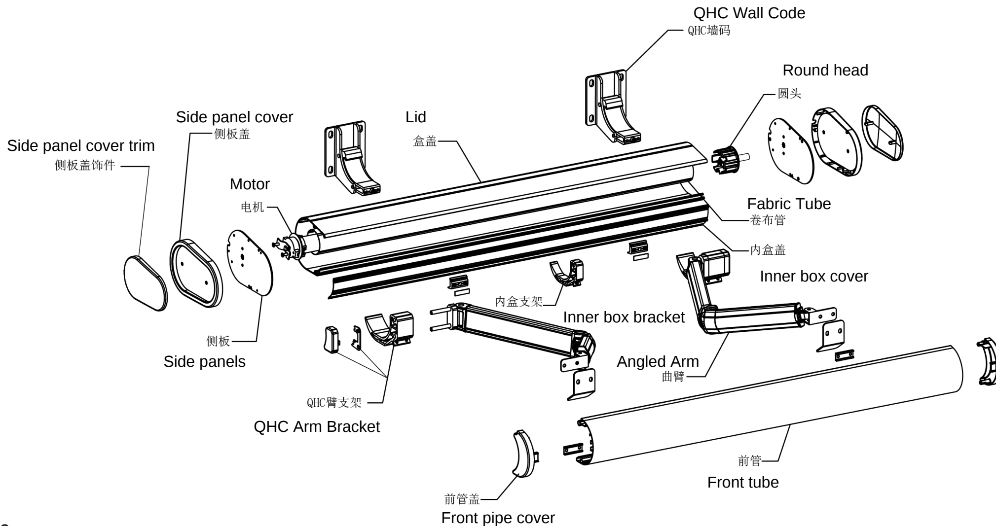
Product explosion diagram
